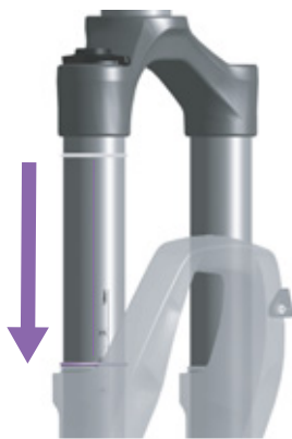
Figure 131: Moving the O-ring on the suspension fork
