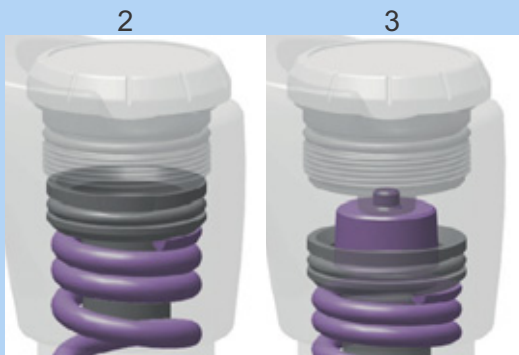
Figure 129: Screwing and unscrewing the preload adjustment ring
