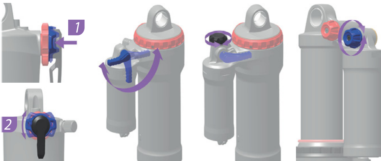
Figure 286: Position and shape of the compression adjuster (blue) depends on the model
