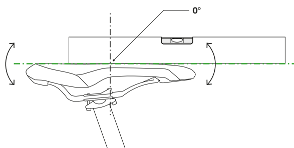
Figure 104: Horizontal saddle tilt with 0° tilt in the centre of the saddle
