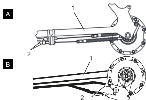
Figure 190: Adjusting sleeves (2) on two alternative versions (A and B) of a dual-cable, Bowden-cable-operated gear shift on the chain stay (1)
