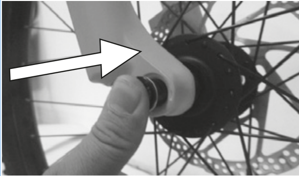
Figure 70: Inserting the axle in the direction of the arrow
