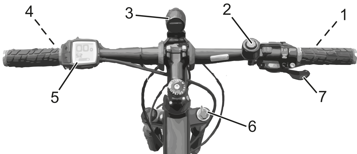
Figure 44: Detailed view of handlebars from sitting position, example
