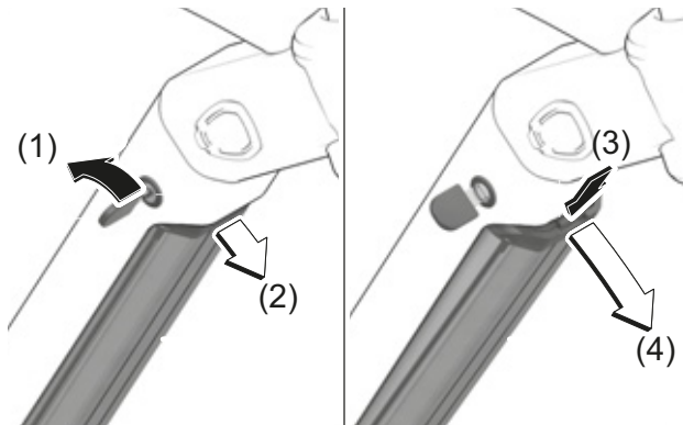
Figure 163: Removing the integrated battery
