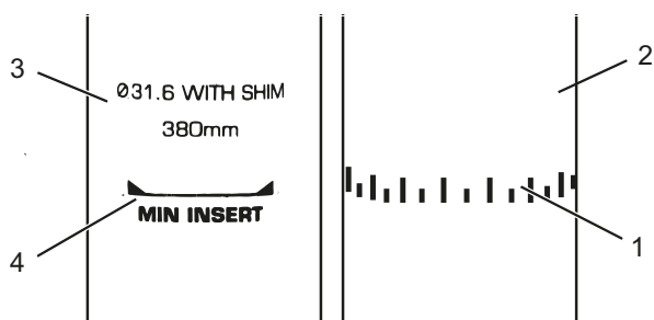
Figure 92: Detailed view of the seat post – examples of the minimum insertion depth marking
