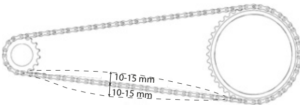
Figure 186: Checking the chain tension
