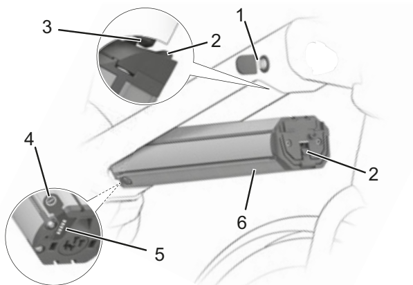
Figure 42: Integrated battery in detail
