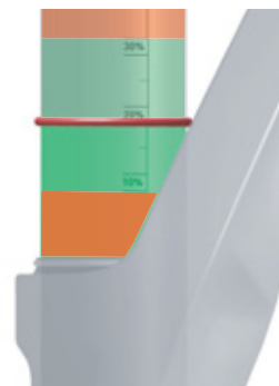
Figure 136: Mandatory sag range (green) and prohibited sag range (red)
