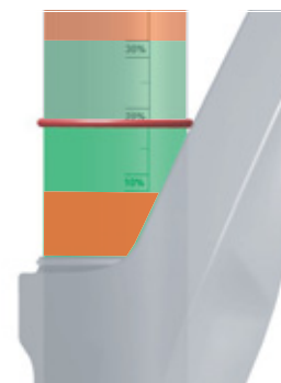
Figure 133: Mandatory sag range (green) and prohibited sag range (red)
