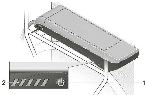
Figure 50: Position of charge level indicator on pannier rack battery
