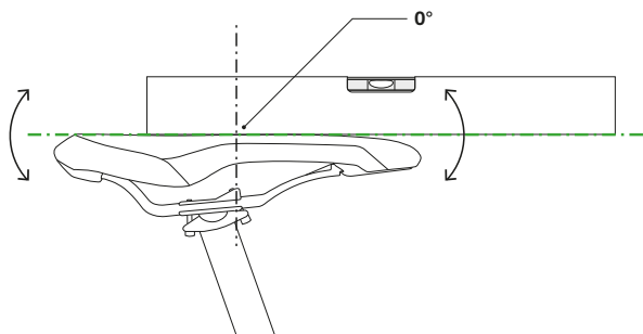
Figure 98: Horizontal saddle tilt with 0° tilt in the centre of the saddle
