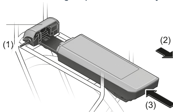
Figure 162: Removing (2) and inserting (3) the pannier rack battery
