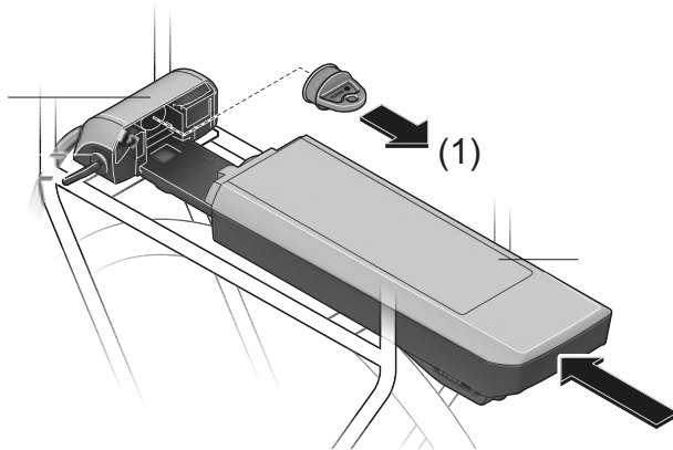
Figure 165: Covering open contacts with cover cap – example: pannier rack battery
