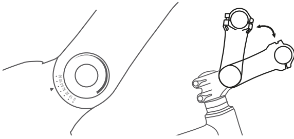
Figure 113: Different versions of angle-adjustable stems
