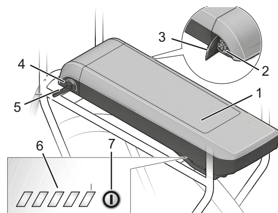
Figure 40: Details of pannier rack battery
