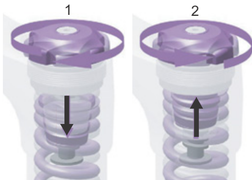
Figure 130: Screwing (1) and unscrewing (2) the preload adjustment ring.
